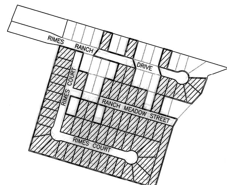
KEY PLAN The Shaded lots are being amended due to the fact that curve data was omitted from original Final Plat.
