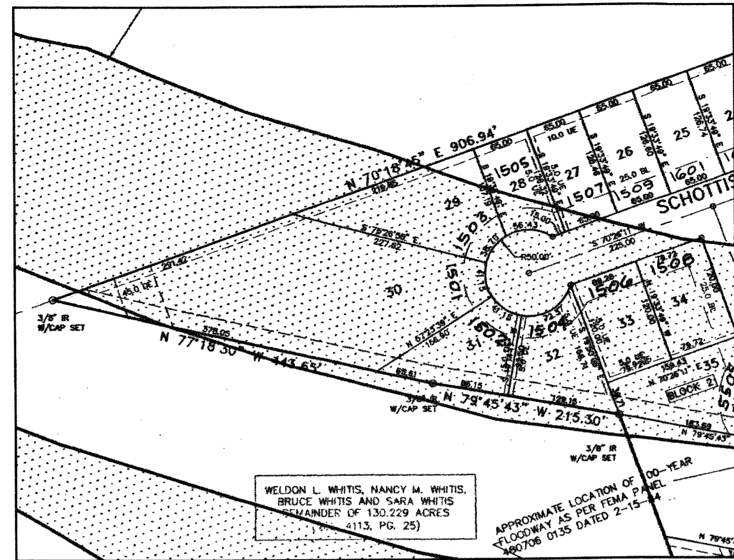
INSET "A" SAEGERT RANCH, PHASE ONE SCALE: 1" = 100'
